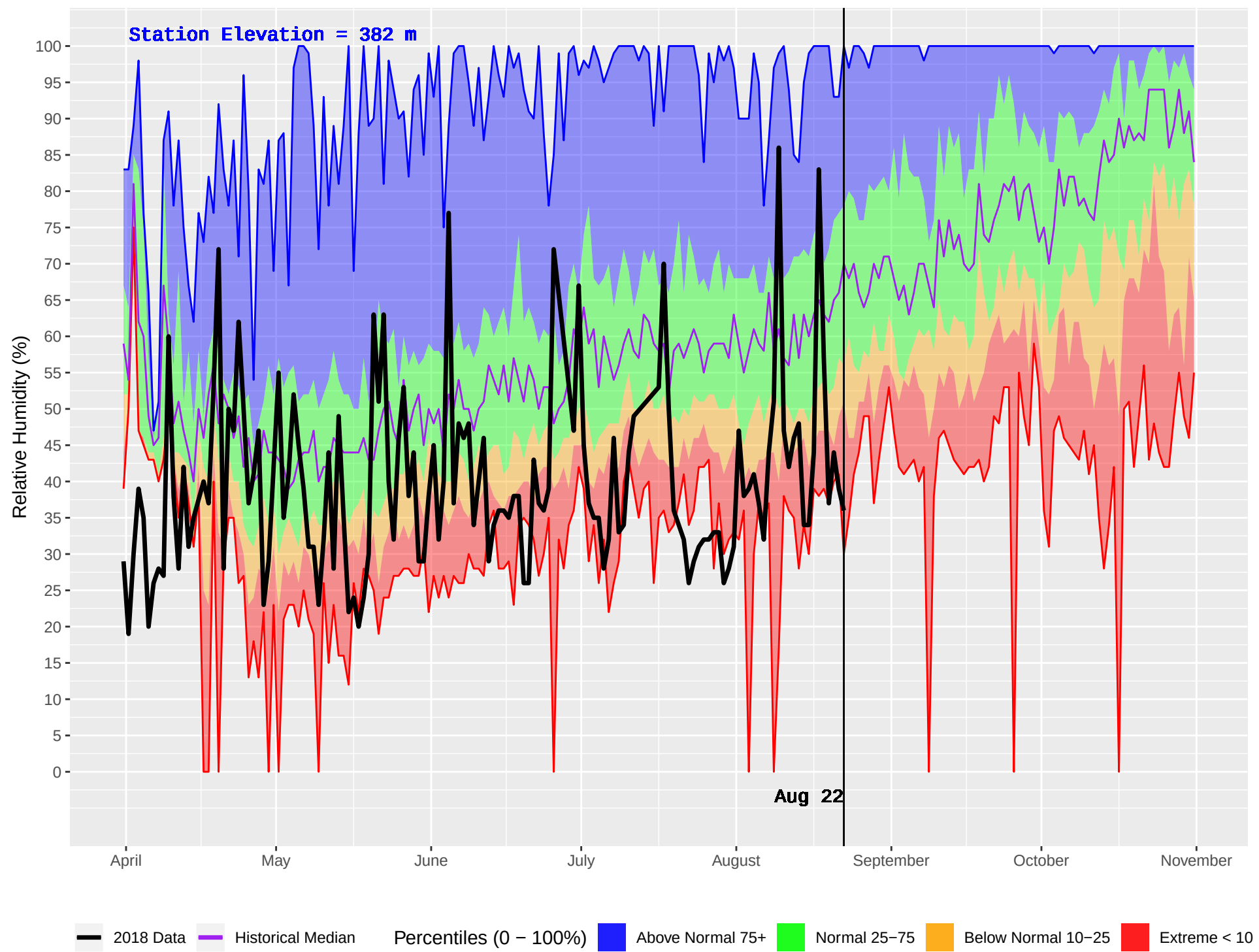
TELEGRAPH CREEK (110) : Historical (1978–2016) and Current (2018) Daily Relative Humidity
