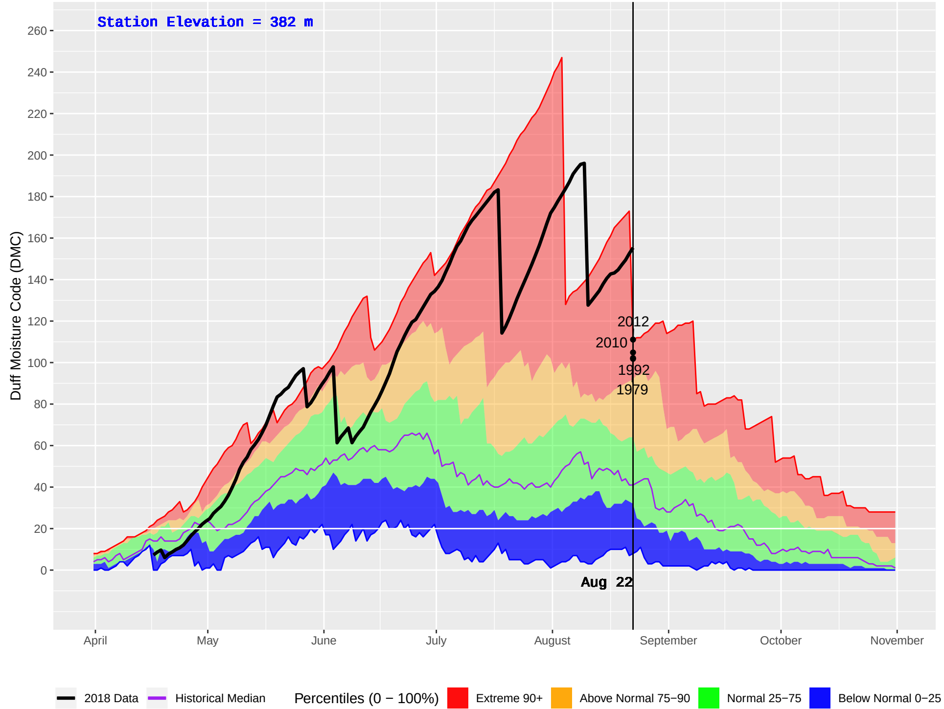
TELEGRAPH CREEK (110) : Historical (1978–2016) and Current (2018) Daily Duff Moisture Code (DMC)
