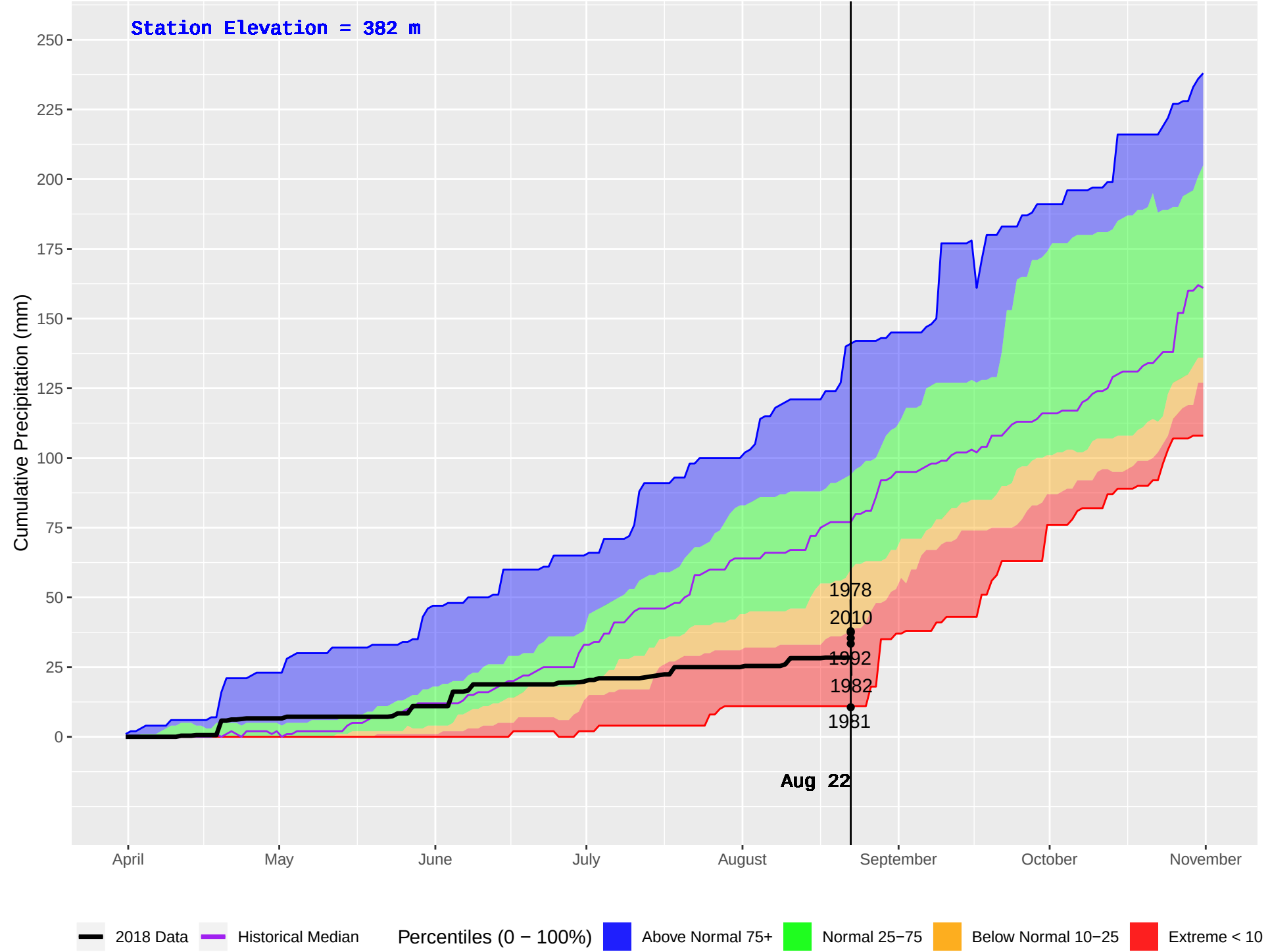
TELEGRAPH CREEK (110) : Historical (1978–2016) and Current (2018) Daily Cumulative Precipitation
