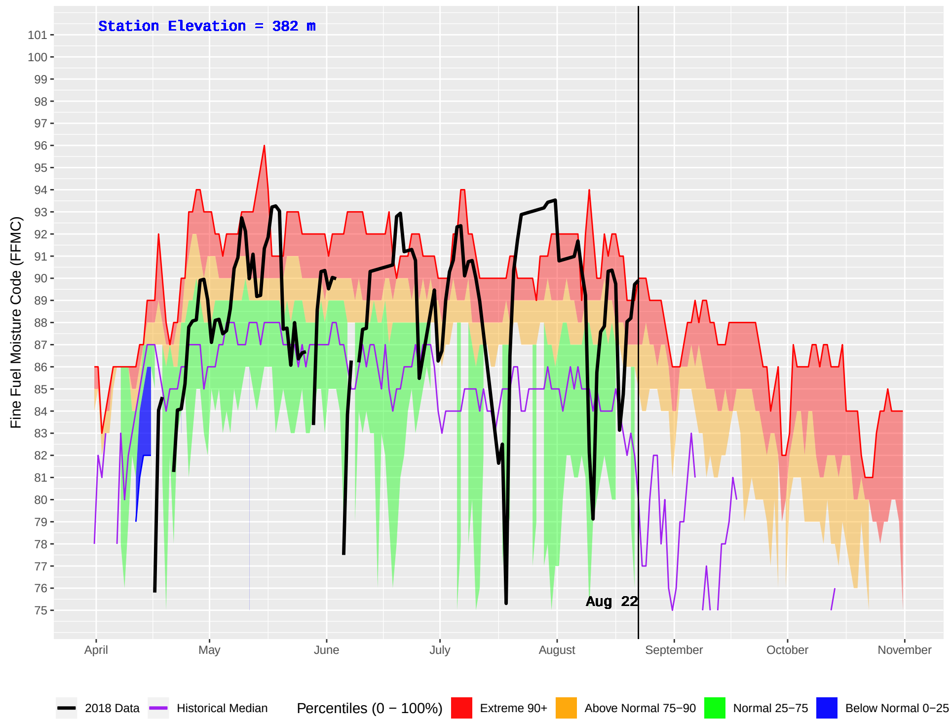
TELEGRAPH CREEK (110) : Historical (1978–2016) and Current (2018) Daily Fine Fuel Moisture Code (FFMC)
