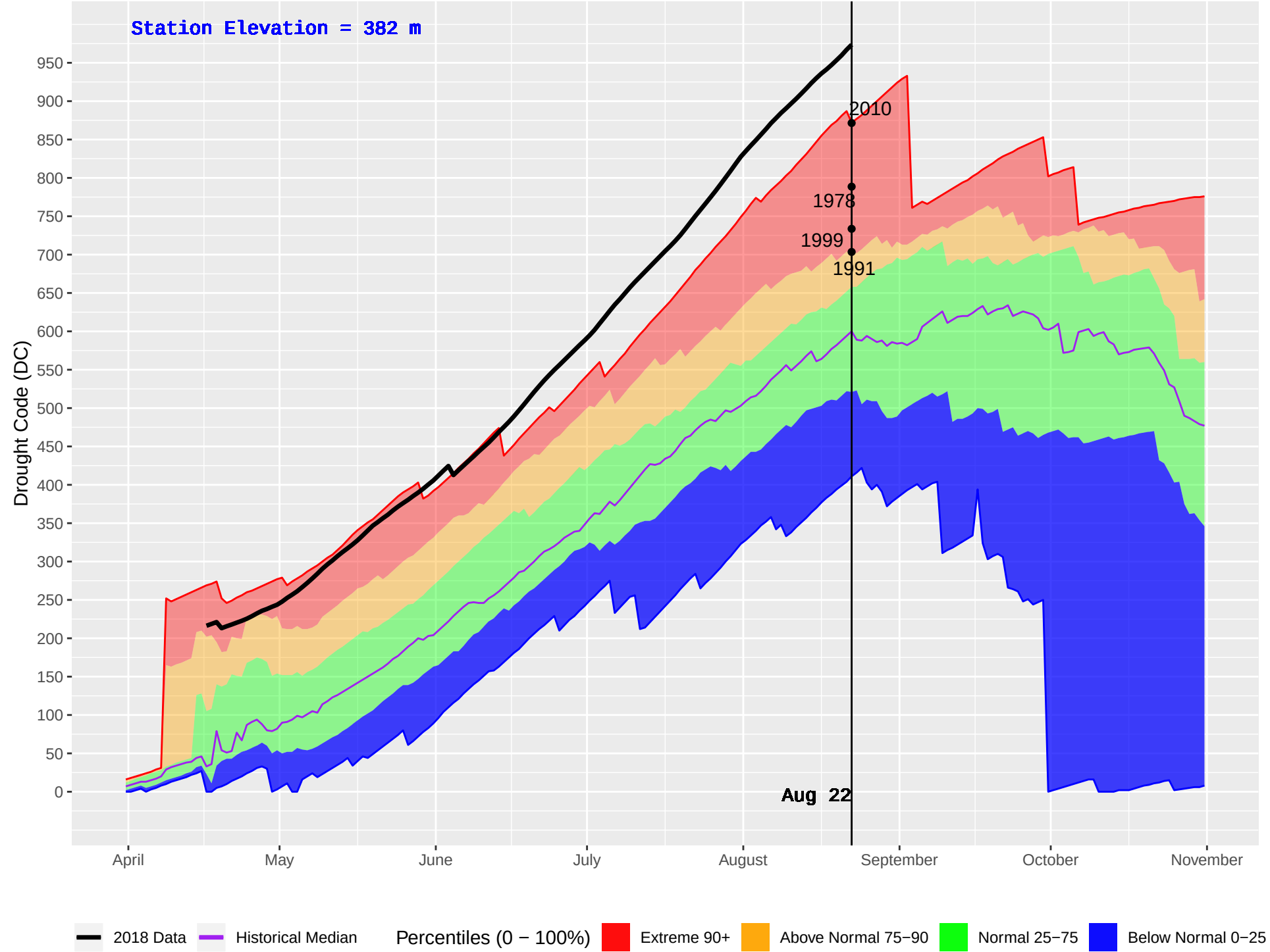
TELEGRAPH CREEK (110) : Historical (1978–2016) and Current (2018) Daily Drought Code (DC)
