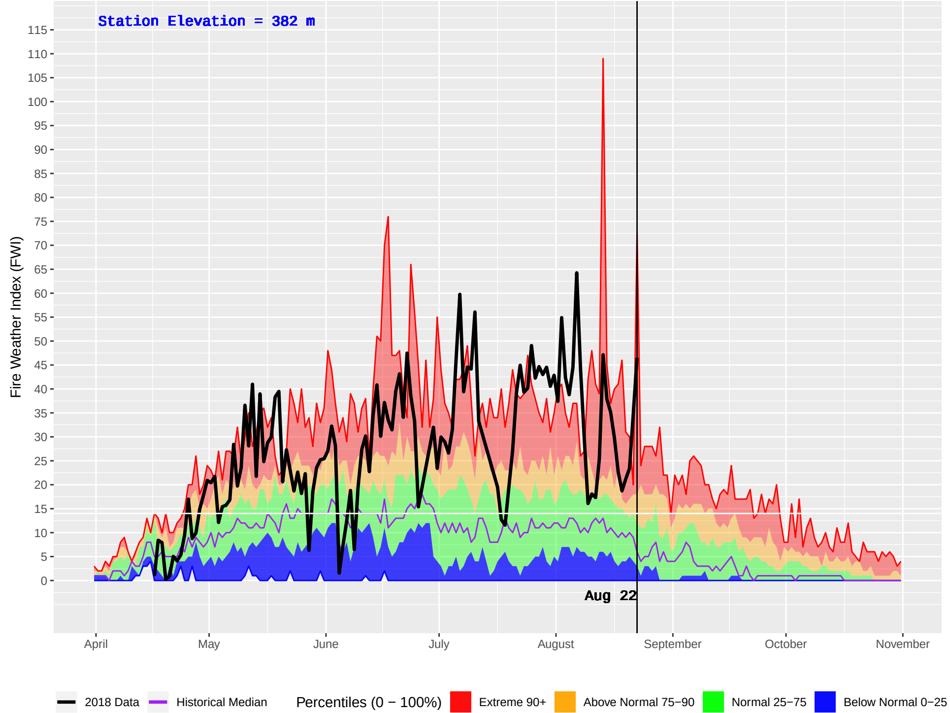
TELEGRAPH CREEK (110) : Historical (1978–2016) and Current (2018) Daily Fire Weather Index (FWI)
