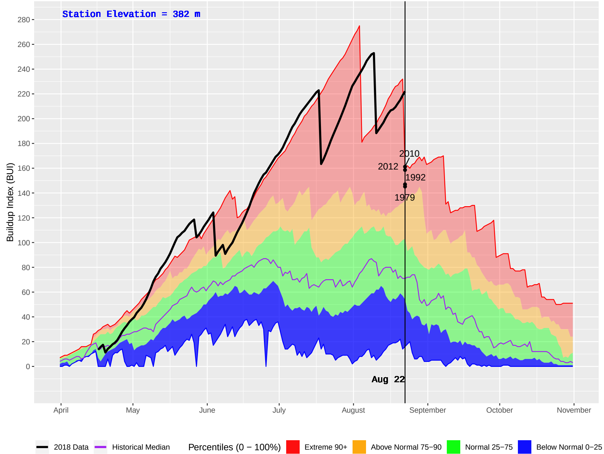
TELEGRAPH CREEK (110) : Historical (1978–2016) and Current (2018) Daily Buildup Index (BUI)
